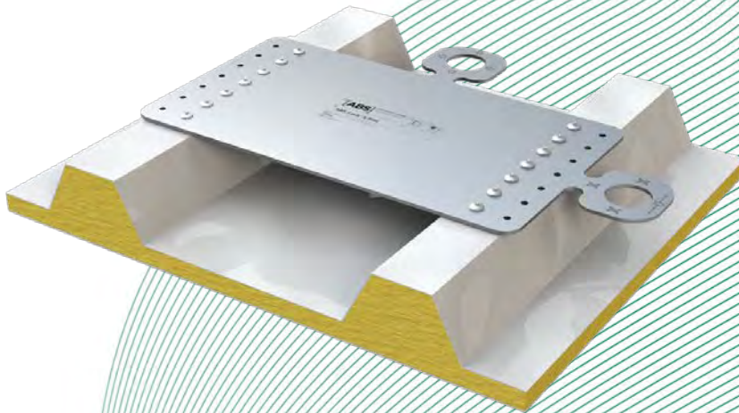
Fig. 1: Anchor device, type: ABS-Lock® X-Flat (riveted)
