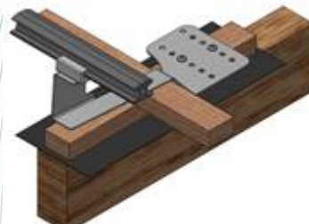
Fig. 6: Rail with bracket for steep roofs
